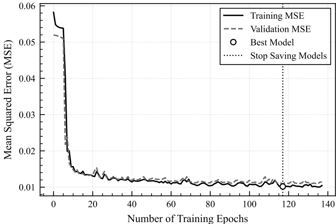
Learning Curve of TCSA-GRU Model for SolarPlant-1 (Gyeongju)
